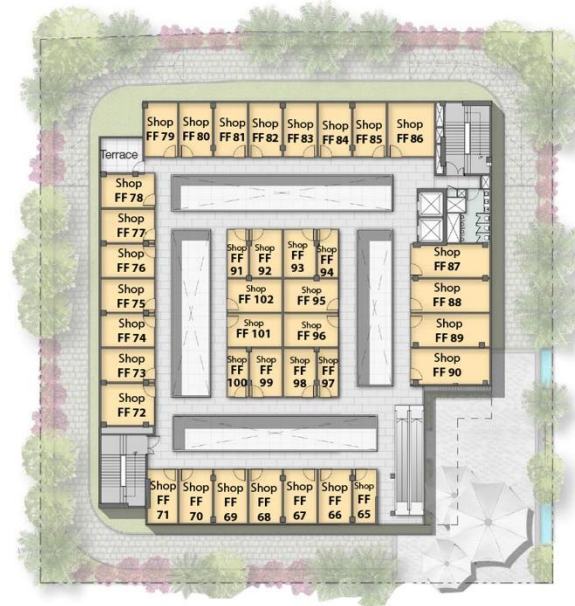
FIRST FLOOR PLAN COMMERCIAL DEVELOPMENT AT SECTOR 50, GURUGRAM
